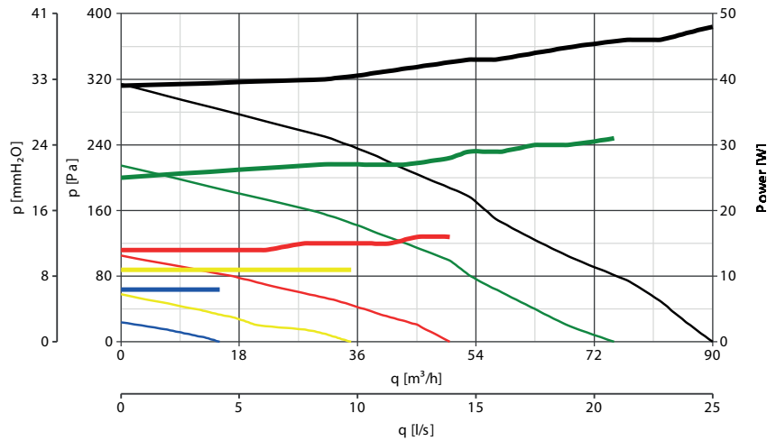
VORT HR W-ALL 100 DF SR COD. 12485 (SEMI-RECESSED INSTALLATION)
